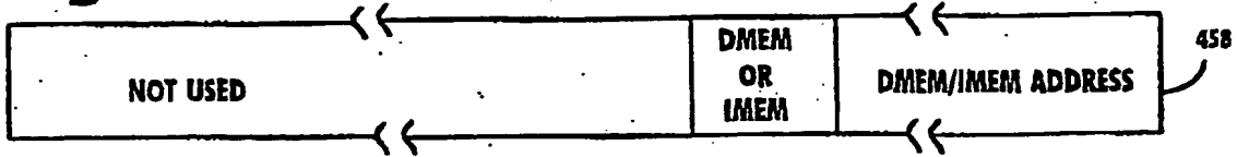
Fig. 7C SP DRAM DMA ADDRESS REGISTER (R/W)
